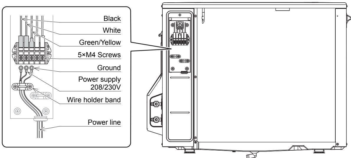
Figure 5: Connect power
