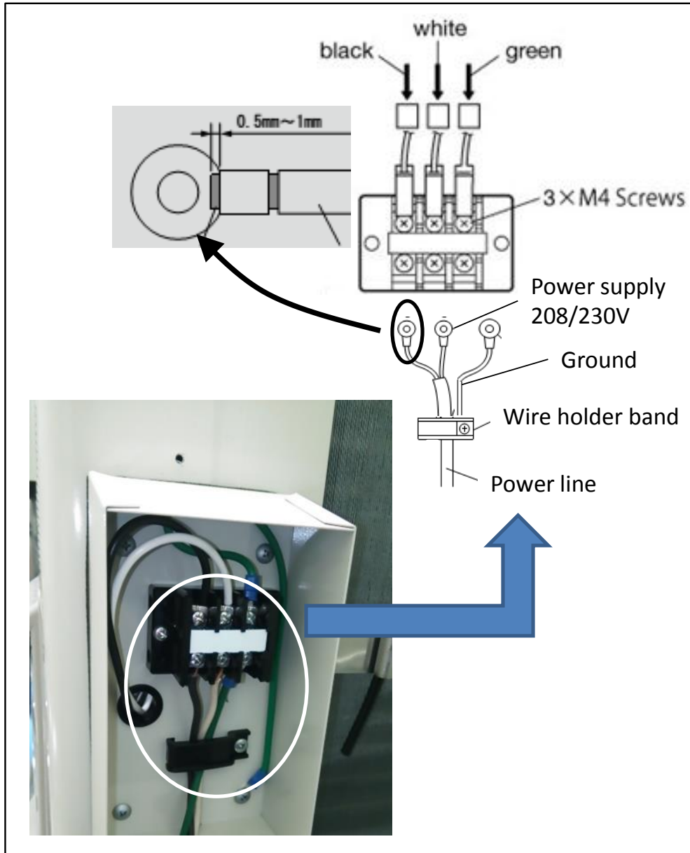
Figure 5: Power connection
