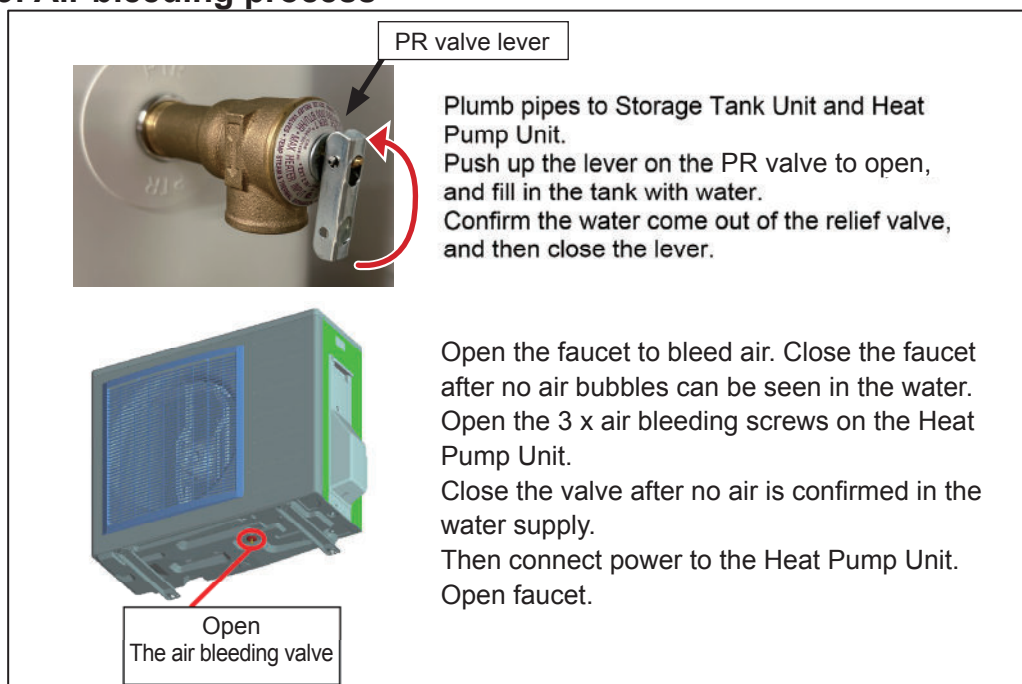
Figure 3: Air bleeding process
