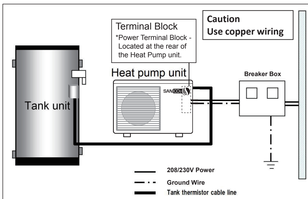
Figure 5: Outline of electrical system connections
