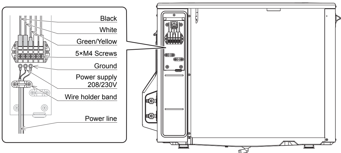
Figure 4: Connect power
